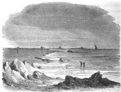
FIELD ICE.
