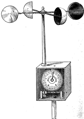
THE ANEMOMETER.
