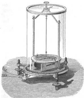
THE TORSION BALANCE.
