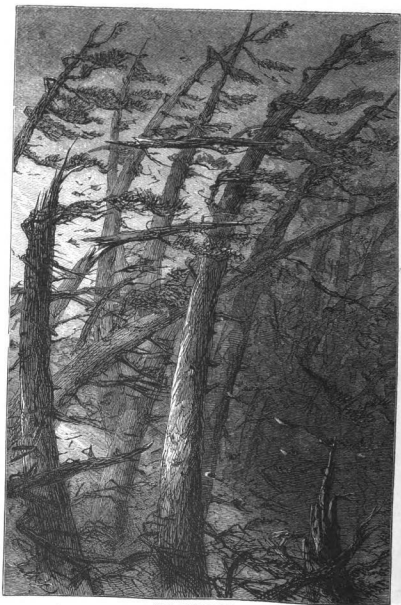
THE HURRICANE.
