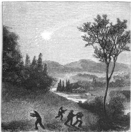
THE METEOR.
