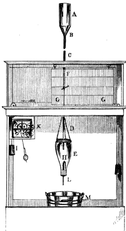
SELF-REGISTERING PLUVIAMETER.
